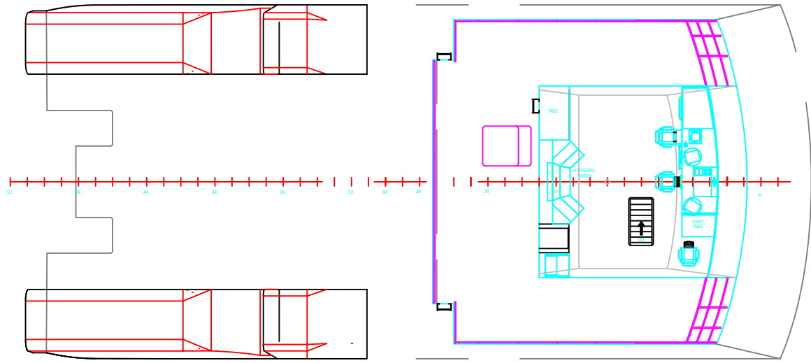
PLAN AT 02 DECK
